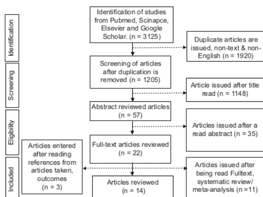
Figure 1: Flowchart literature
